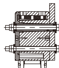
Side connection
