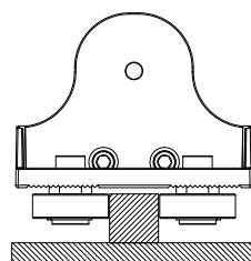
Guide rollers/fittings HWS112-HWS200
